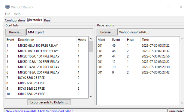
Fig. 2: Directories tab
